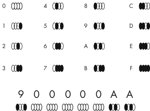
Figure 2-2: A hexadecimal font
